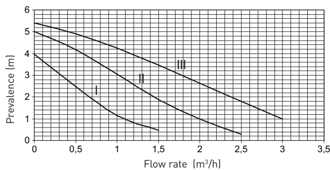
PREVALENCE FOR THE THREE SPEEDS OF THE WILO ST 15/6 ECO SOLAR PUMP
